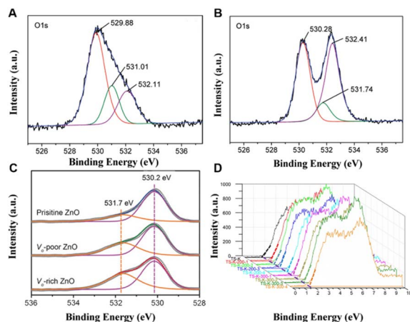
Fig. 10 (A) XPS of pure \text{TiO}_2 nanorods and (B) \text{TiO}_2 nanorods with Cu doping. 110 Copyright © 2010 American Chemical Society. (C) XPS of \text{V}_o -rich ZnO. 112 Copyright © 2012 American Chemical Society. (D) XPS valence band spectra of black \text{TiO}_2 samples. 113 Copyright © 2018 Elsevier Inc.
