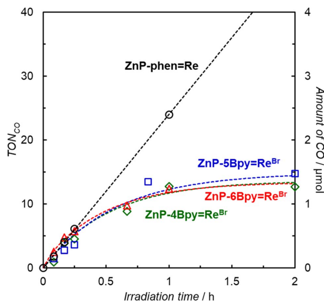
Fig. 7 Time dependence of CO formation (0–2 h) during irradiation at 420 nm by LED lamps (input power: 30 mW), in a merry-go-round irradiation apparatus, of CO 2 -saturated DMA solutions containing the dyad (0.05 mM) and BIH (0.05 M).
