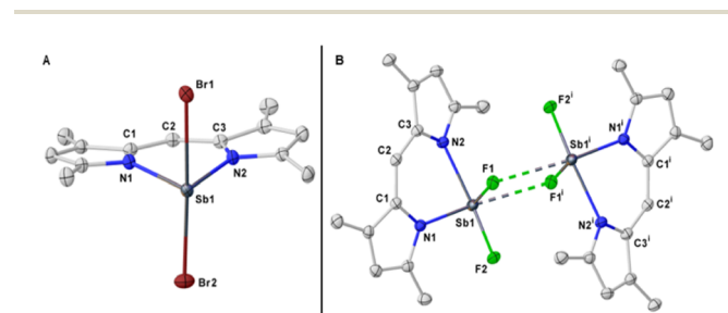
Fig. 5 (A) Single crystal X-ray of complex SBDIPY-1-Br; (B) SBDIPY-1-F. Displacement ellipsoids are drawn at 50% probability level; hydrogen atoms are omitted for clarity.
