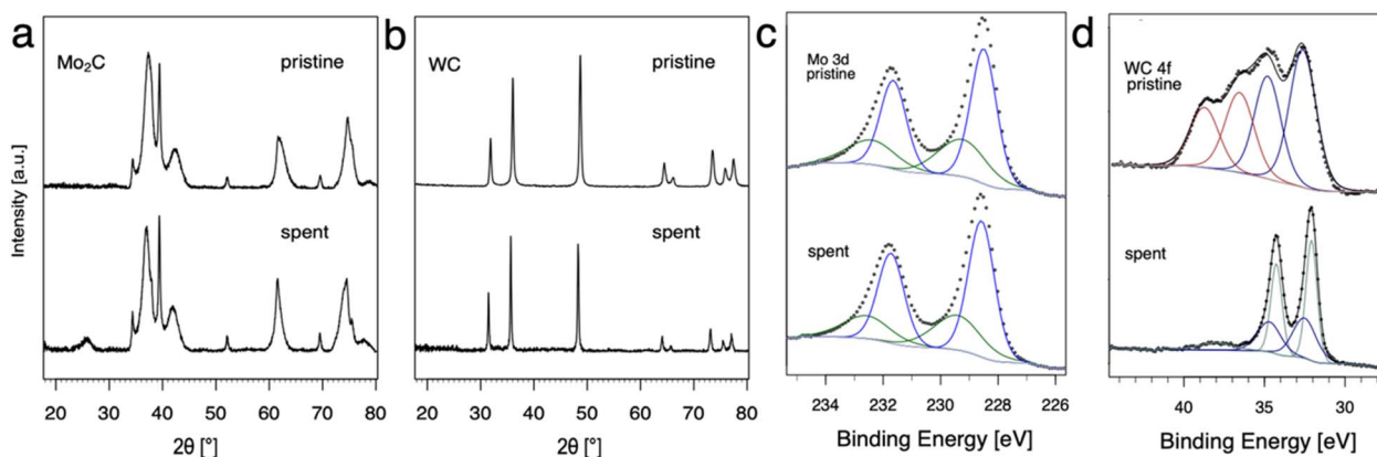
Fig. 2 Structural transformations for pristine and spent catalyst materials are shown. pXRD for (a) \text{Mo}_2\text{C} , (b) WC and XPS spectra of pristine and spent metal carbides: (c) \text{Mo}_{2\text{C}} 3d, (d) WC 4f. The dots represent the recorded data and the solid lines show the results of a curve-fitting procedure.
