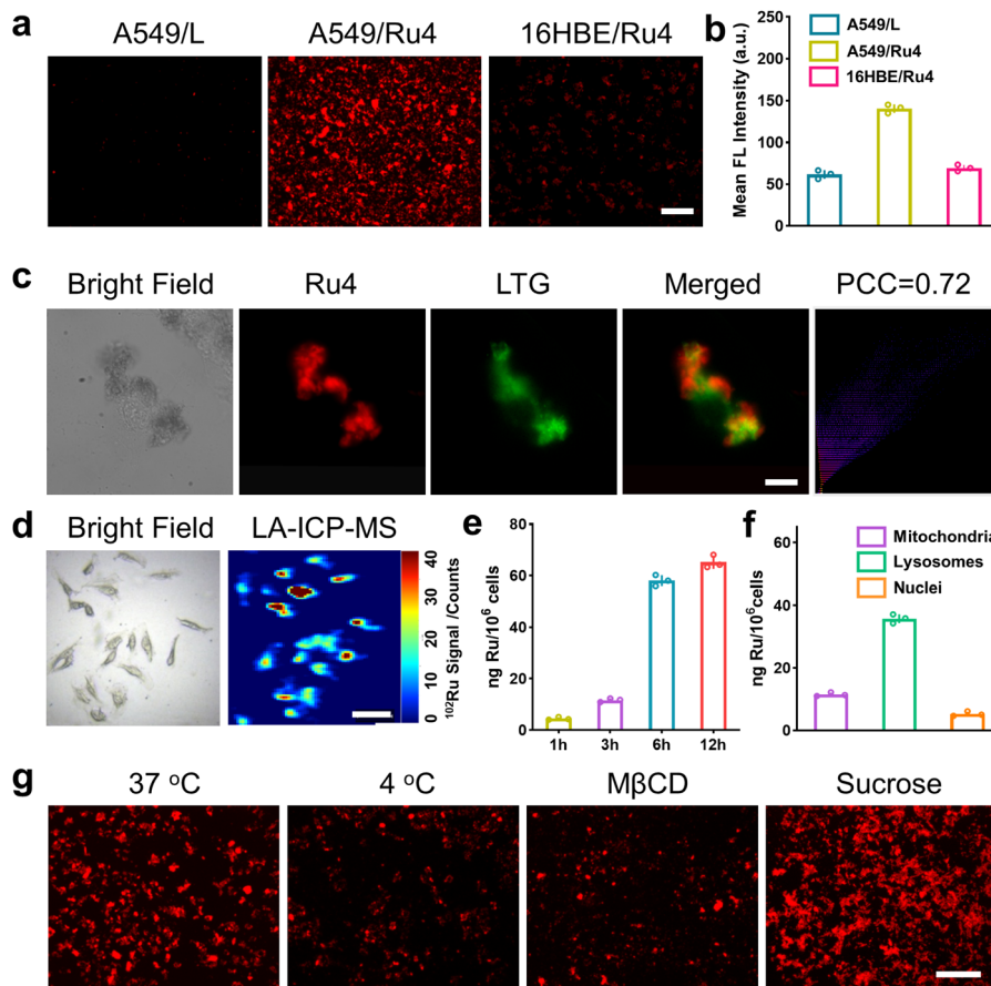
Fig. 4 Cellular uptake and localization of Ru4 in A549 cells. (a) Fluorescence images of cells treated with Ru4 (10 μM) and L (20 μM), respectively. Scale bar: 300 μm. (b) Semi-quantitative analysis of the fluorescence imaging in Fig. 4a. (c) Colocalization assay of Ru4 (10 μM) using LTG. Scale bar: 10 μm. (d) LA-ICP-MS imaging of 102 Ru in A549 cells incubated with Ru4 (10 μM). Scale bar: 50 μm. (e) ICP-MS results showing the Ru content in A549 cells over time. (f) Subcellular distribution of Ru concentration in A549 cells measured using ICP-MS. (g) Cellular uptake mechanism studies of Ru4 (10 μM) at 4 °C and 37 °C, MβCD and sucrose, respectively. Scale bar: 300 μm.
