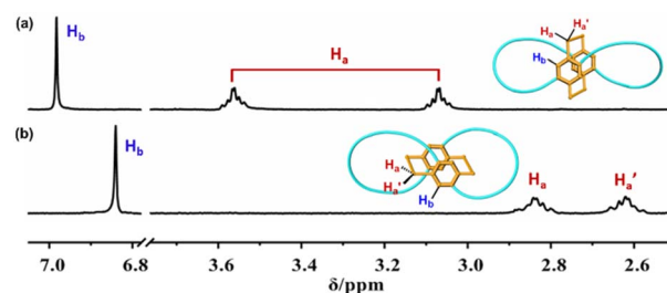
Fig. 3 Comparison of the ^1\text{H} NMR spectra (600 MHz, \text{CDCl}_3 , 298 K) of (a) bis-po-CC and (b) bis-pm-TC .
