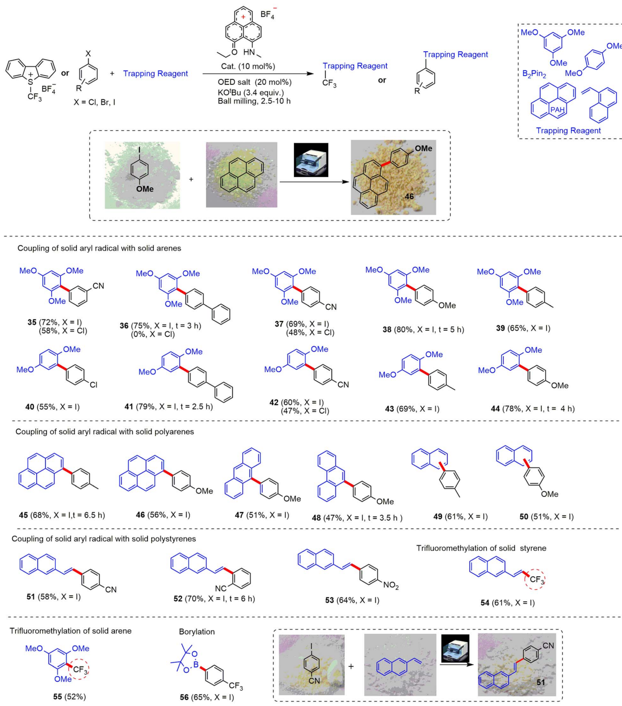
Fig. 4 Substrate scope of solid–solid coupling reactions. Reaction conditions: aryl halide (0.3 mmol), styrene (3.5–5 equiv.), PLY I (10 mol%), OED salt 20 mol%, KO t Bu 3.4 equiv., LAG (DMSO, 0.12 \mu\text{L mg}^{-1} ), ball milling, unless otherwise specified, the reaction time is 10 h.
