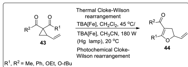
Scheme 15 Synthesis of substituted vinylidihydrofurans 44 via Cloke–Wilson rearrangement.
