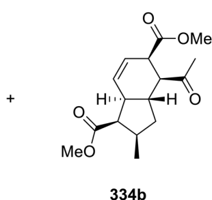
Scheme 44 Synthesis of hydrindanes 334.
