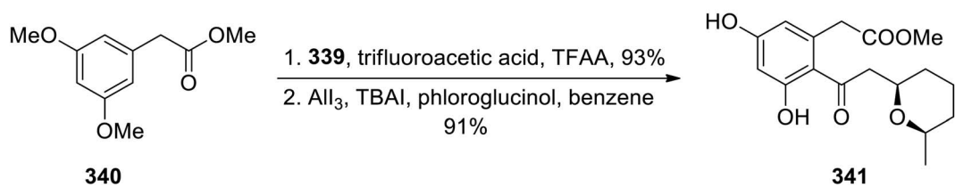
Scheme 45 Synthesis of curvulone B 341.
