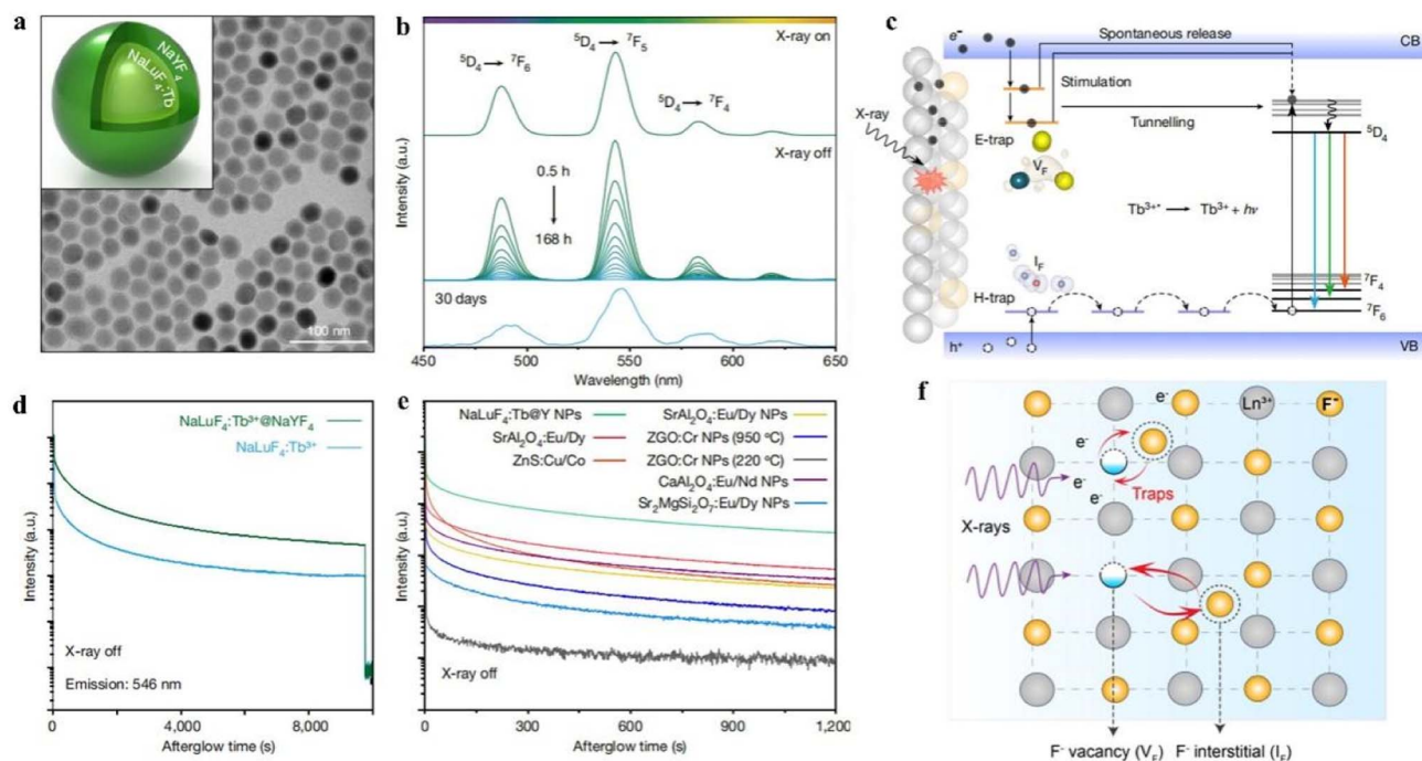
Fig. 6 (a) TEM images of NaLuF 4 :Tb@NaYF 4 NPs; (b) radioluminescence emission spectra of NaLuF 4 :Tb@NaYF 4 NPs after 50 kV stop X-ray irradiation for 0.5–168 h or 30 days; (c) mechanism of sustained luminescence of Tb 3+ -doped NaLuF 4 NPs; (d) variation of radioluminescence intensity with time for NaLuF 4 :Tb and NaLuF 4 :Tb@NaYF 4 nanocrystals at 546 nm as a function of time; (e) afterglow decay curves of different phosphors after 50 kV X-ray excitation; (f) generation of Frenkel trap states in NaLuF 4 lattice under X-ray irradiation. The small fluoride ions (F - ) then migrate from the lattice to the interstitial sites. This leads to the production of many fluoride vacancies (V F ) and interstitials (I F ) and is accompanied by the capture of high-energy electrons (e - ) at the defects. 28
