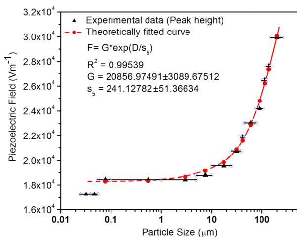
Fig. 7 Variation of piezoelectric field with the particle size of the SAOE ML phosphor material. The data has also been fitted theoretically to see the trend and it is shown in the inset. It is observed that there is a very good correlation between the piezoelectric field and the particle size. It could be seen that the piezoelectric constant decreases exponentially with the particle size decreasing. The formulation used for fitting is also given in the inset.
