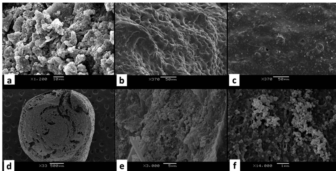
Fig. 3 Scanning electron micrograph of (a) starting biomaterial used to form the hydrogel beads from the treatment of switchgrass, (b) surface of freeze-dried hydrogel bead based on switchgrass biomaterial, (c) surface of hydrogel based on switchgrass with entrapped laccase, (d) a cross-section of the bead of hydrogel with entrapped laccase, (e and f) magnification of the cross section shown in (d).
