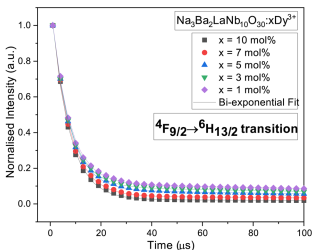
Fig. 19 Decay curves for 4F_{9/2} \rightarrow 6H_{13/2} transition in \text{Na}_3\text{Ba}_2\text{LaNb}_{10}\text{O}_{30}:\text{x}\text{Dy}^{3+} ( x = 1, 3, 5, 7 and 10 mol%) phosphors.
