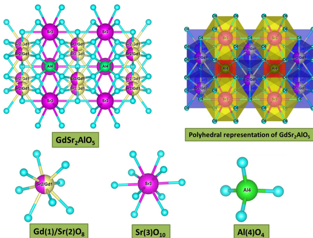
Fig. 3 3-D structural view of host GdSr _2 AlO _5 sample along with coordinative environment of different cations.
