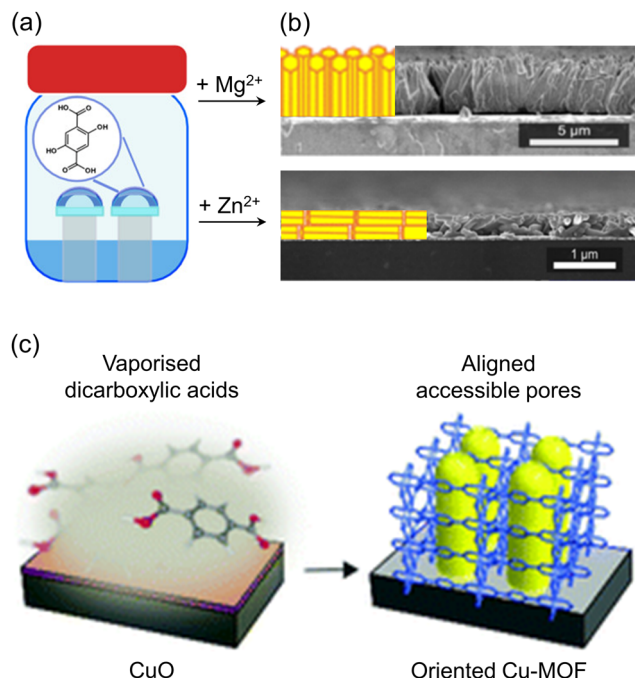
Fig. 10 (a) Schematic illustration of VAC reactions for MOF-74 films with Mg^{2+} or Zn^{2+} as a metal source. (b) Cross-sectional SEM images of Mg-MOF-74 film (top) and Zn-MOF-74 film (bottom). Adapted with permission from ref. 88. Copyright 2021, American Chemical Society. (c) Schematic illustration of the CVD process for synthesizing oriented films of CuCDC and CuBDC by reacting a deposited layer of CuO with a vaporized carboxylic acid. Adapted with permission from ref. 89. Copyright 2019, Royal Society of Chemistry.
