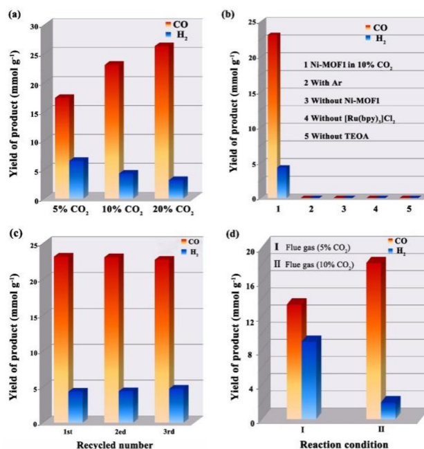
Fig. 3 \text{CO}_2 photoreduction performance and recycling. (a) Ni-MOF1 under different \text{CO}_2 concentrations. (b) Ni-MOF1 under various reaction conditions. (c) Cycling tests under 3 h of irradiation in a 10% \text{CO}_2 atmosphere over Ni-MOF1. (d) The yield of CO and \text{H}_2 on Ni-MOF1 in real flue gas.
