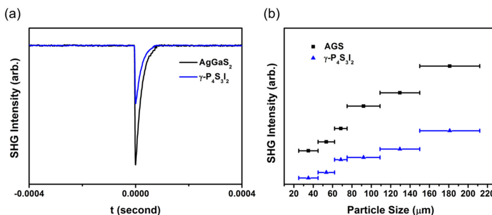
Fig. 3 Measured SHG signals of \gamma\text{-P}_4\text{S}_3\text{I}_2 and \text{AgGaS}_2 with a 150–210 \mu\text{m} particle size (a). Measured SHG intensities of \gamma\text{-P}_4\text{S}_3\text{I}_2 and \text{AgGaS}_2 under 2.05 \mu\text{m} laser irradiation at room temperature (b).
