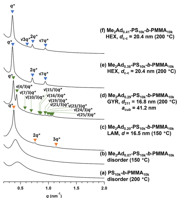
Fig. 8 SAXS profiles of thermally annealed Me 2 Ad-PS 10k -b-PMMA 10k . (a) PS 10k -b-PMMA 10k , (b) Me 2 Ad 0.07 -PS 10k -b-PMMA 10k , (c) Me 2 Ad 0.20 -PS 10k -b-PMMA 10k , (d) Me 2 Ad 0.29 -PS 10k -b-PMMA 10k , (e) Me 2 Ad 0.38 -PS 10k -b-PMMA 10k and (f) Me 2 Ad 0.41 -PS 10k -b-PMMA 10k . The value in the parentheses represents the annealing temperature.
