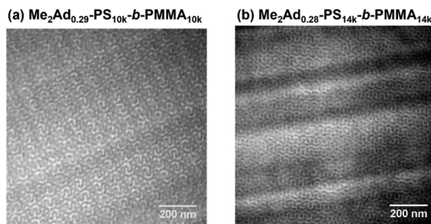
Fig. 9 TEM micrographs of (a) Me 2 Ad 0.29 -PS 10k -b-PMMA 10k (annealed at 200 °C for 24 h) and (b) Me 2 Ad 0.28 -PS 14k -b-PMMA 14k (annealed at 250 °C for 24 h).
