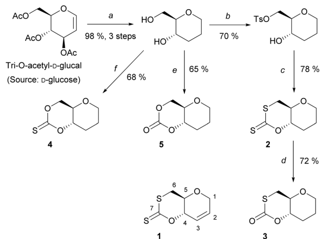
Scheme 1 Synthesis of monomers, 1–5, from tri- O -acetyl- D -glucal; (a) (i) Et 3 SiH, BF 3 ·OEt 2 , DCM, 0 °C, 3 h, (ii) NaOMe (cat.), MeOH, rt, 2 h, (iii) Pd/C, MeOH, rt, 20 h (98%, 3 steps); (b) TsCl, pyridine, rt, 20 h, 70%; (c) CS 2 , t -BuOK, THF, 0 °C, 3 h, 78%; (d) O 3 , DCM, -78 °C, 72%; (e) CDI, DCM, 0 to 20 °C, 3 h, 65%; (f) TCDI, DCM, 0 to 20 °C, 3 h, 68%. Monomer 1 was synthesised according to literature. 21
