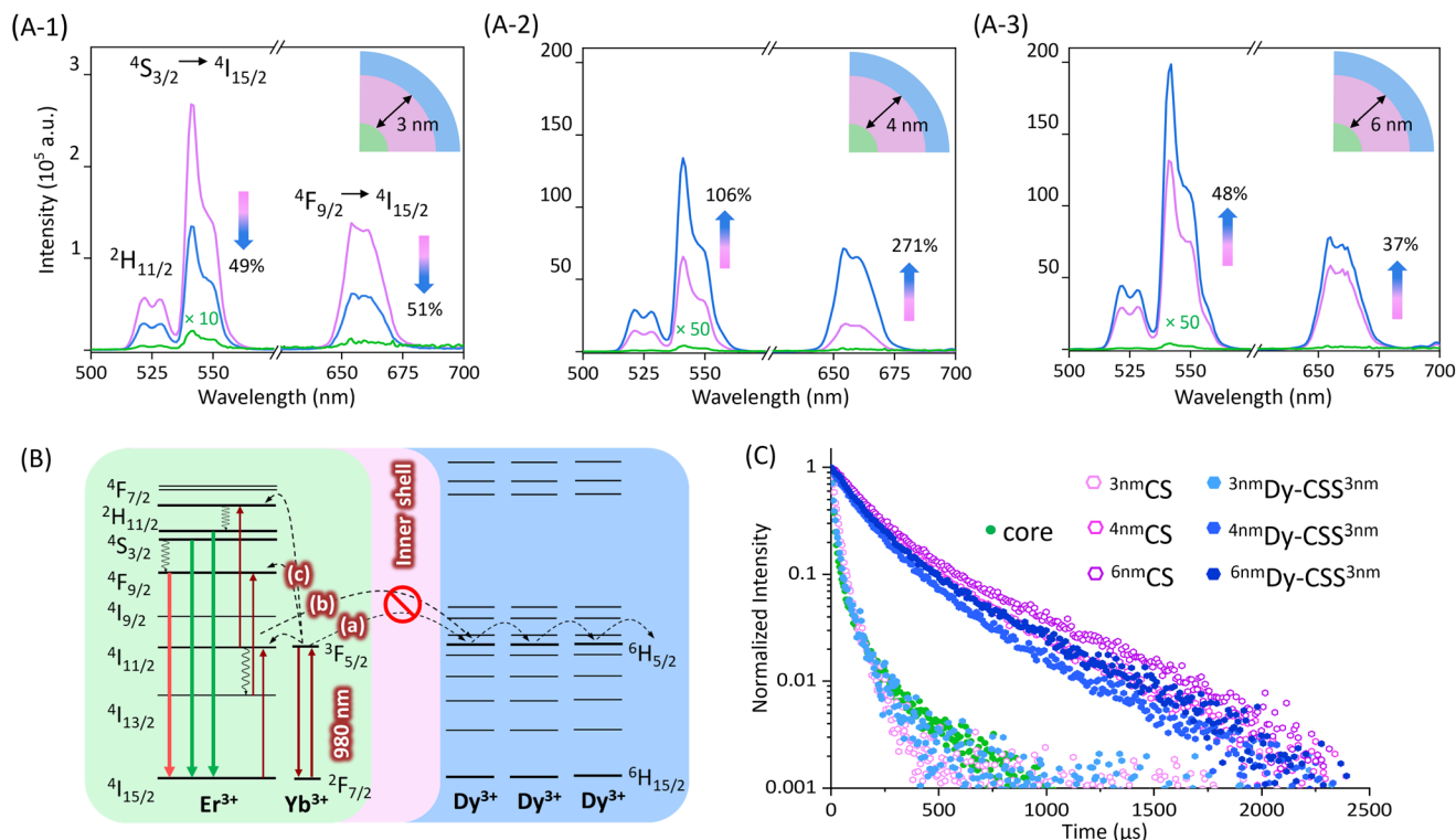
Fig. 2 (A) UC spectra of OA-capped 3 nmDy-CSS 3 nm (1), 4 nmDy-CSS 3 nm (2), and 6 nmDy-CSS 3 nm (3) NPs (blue) as well as their corresponding core (green) and CS (pink) NPs. All spectra were obtained under 980 nm laser excitation. Power density = 6.0 W cm -2 , [NP] = 5 mg mL -1 in toluene. (B) Partial energy level diagram for Er 3+ /Yb 3+ and Dy 3+ , schematically showing how the addition of an inner shell physically separates Er 3+ /Yb 3+ from Dy 3+ ions, thus, preventing Dy 3+ -induced loss of the UC. Solid lines are radiative transitions, dotted lines indicate energy transfer, and wavy lines are non-radiative transitions. (C) Luminescence decay curves of the Yb 3+ emission under 980 nm excitation obtained from core, CS, and CSS NPs.
