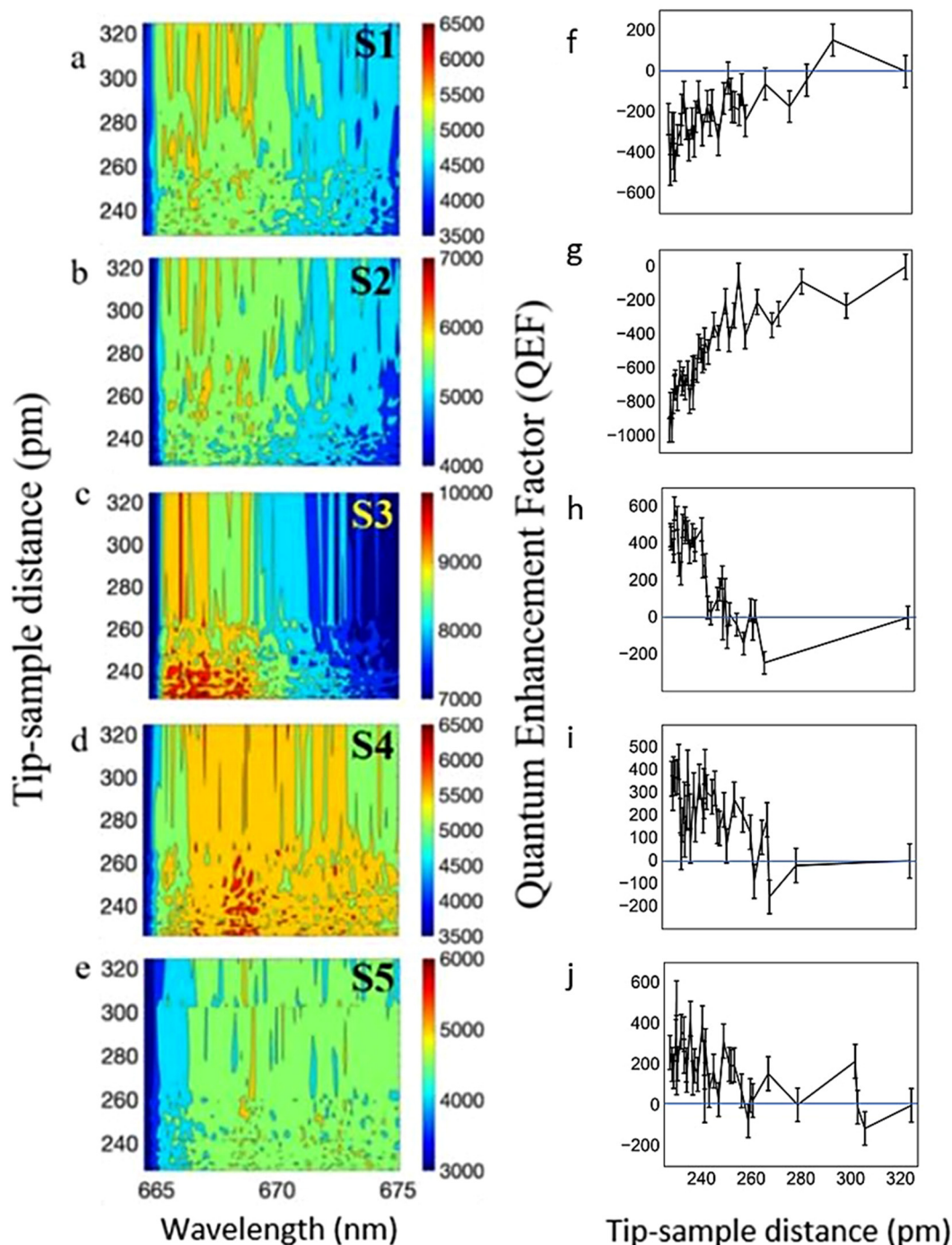
Fig. 3 Picoscale TSD dependent PL of WS 2 -MoS 2 lateral heterostructure in the quantum tunneling regime. (a–e) 2D contour plots and (f–j) quantum enhancement factors for the locations S1–S5 corresponding to Fig. 2.
