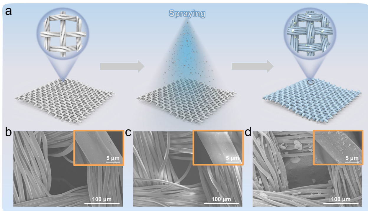
Fig. 3 Preparation illustration of a conductive curtain containing photocatalyst. (a) Preparation illustration of a conductive curtain containing g-C 3 N 4 /TiO 2 . SEM images of (b) the curtain after pretreatment, (c) conductive curtain, and (d) conductive curtain containing g-C 3 N 4 /TiO 2 , scale bar: 100 μm (inset, scale bar: 5 μm).
