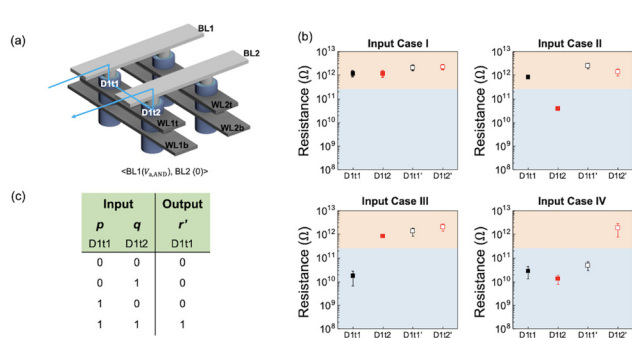
Fig. 5 Experimental demonstration of the AND logic gate between D_{11t} and D_{12t} memristors in the BLC. (a) The bias configuration in the schematic diagram of the vertical CBA, where V_{a,\text{AND}} = +9 V. (b) The results of the AND logic operation in D_{11t} for each input case. A resistance lower than 250 G \Omega is encoded to the "1" state and (c) its truth table of the logic gate.
