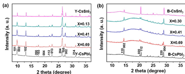
Fig. 7 XRD patterns of (a) Y-phase \text{CsPb}_x\text{Sn}_{1-x}\text{I}_3 NWs and (b) B- \gamma phase \text{CsPb}_x\text{Sn}_{1-x}\text{I}_3 NWs. Reproduced from ref. 78 with permission from the American Chemical Society. Copyright 2018.
