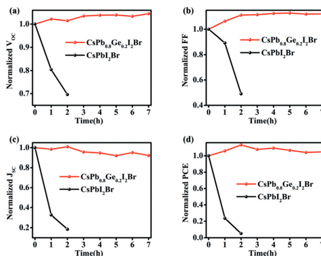
Fig. 8 Stability tests of CsPb 0.8 Ge 0.2 I 2 Br and CsPbI 2 Br PSCs upon the storage in the ambient atmosphere (50--60 % RH): (a) V_{OC} , (b) FF, (c) J_{SC} , and (d) PCE. Reproduced from ref. 80 with permission from Wiley-VCH. Copyright 2018.
