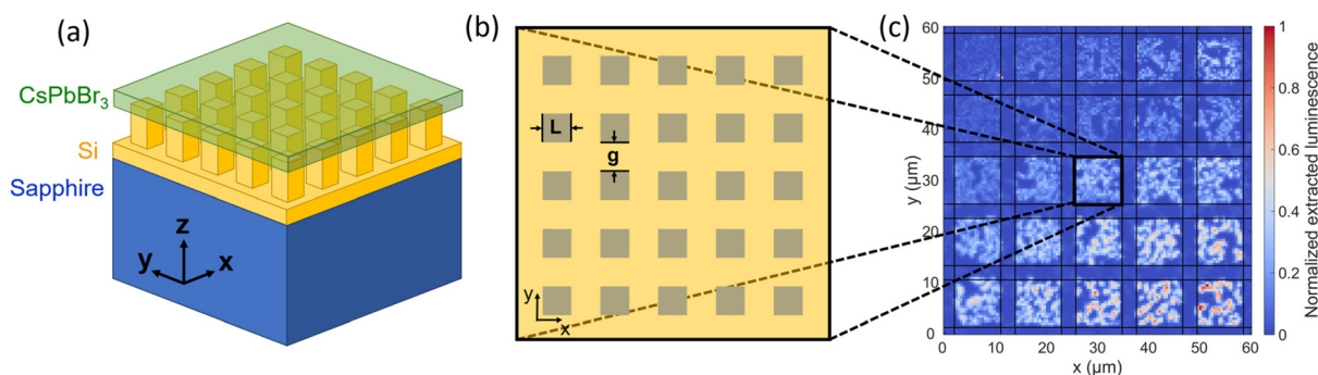
Fig. 1 (a) Schematic representation of the CsPbBr 3 layer deposited on Mie resonators, each corresponding to a set of (L,g) parameters. (b) Geometric parameters defining the size of the square pillars ( L ) and their side-to-side separation, which we refer to as the gap ( g ). (c) Perovskite luminescence, normalized to the maximum intensity of the image, over Mie resonators with varying (L,g) parameters.
