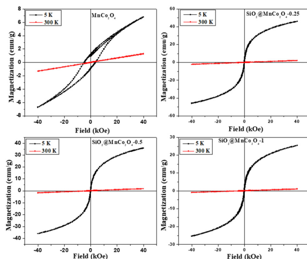
Fig. 5 M - H curves for \text{MnCo}_2\text{O}_4 NPs and \text{SiO}_2@\text{MnCo}_2\text{O}_4 core-shell nanorattles at 300 K and 5 K.
