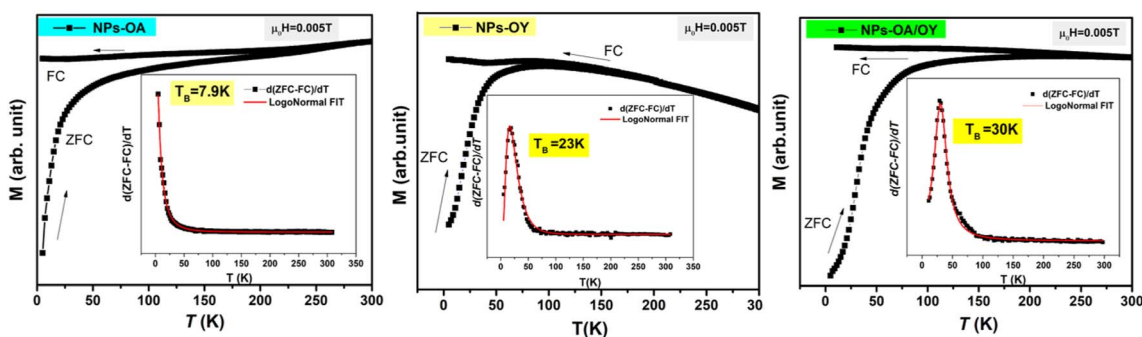
Fig. 5 ZFC/FC magnetization curves and the blocking temperature T_B .
