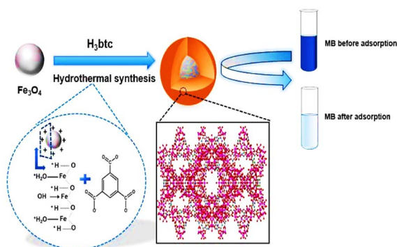
Fig. 7 Schematic representation of the in situ one-step hydrothermal synthesis of Fe 3 O 4 @MIL-100(Fe) core-shell magnetic microspheres (reproduced with permission from ref. 45. Copyright 2017 Elsevier).
