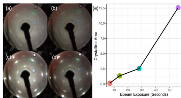
Fig. 4 LEED images showing the spot crystallization obtained after exposing the amorphous Si-on- \text{Ag}(111) surface with a high-energy electron beam ( 2.5\text{ keV} ). The exposure duration is set as follows: (a) 7 seconds, (b) 14 seconds, (c) 28 seconds, and (d) 56 seconds. (e) Is the plot of the nominal crystalline area ( \text{mm}^2 ) with respect to the e-beam exposure duration (a–d). The nominal Si coverage deposited on \text{Ag}(111) was 1.5 monolayers. Black circle \text{Ag}:1 \times 1 spots, (represented once) green: integer order Si spots and blue: \text{Si}:\sqrt{3} \times \sqrt{3} spots with respect to the integer order Si spots inside the green circle. LEED images (a–d) are taken at an incident energy of E_i = 54\text{ eV} .
