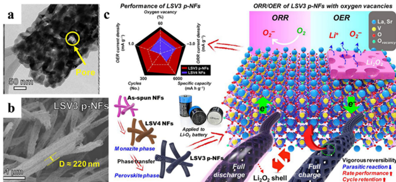
Fig. 13 TEM (a) and SEM (b) of \text{La}_{0.8}\text{Sr}_{0.2}\text{VO}_3 (LSV3 p-NFs). Schematic illustration of LSV3 p-NFs used in rechargeable \text{Li}-\text{O}_2 batteries (c). 136 Copyright © 2020 Elsevier.
