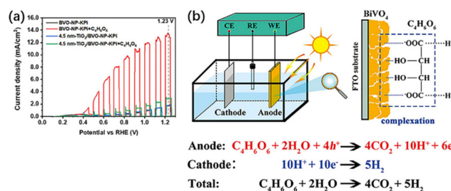
Fig. 7 (a) Current density versus potential curves of BVO-NP and 4.5 nm \text{TiO}_2 /BVO-NP photoanodes in potassium phosphate (KPi) and \text{KPi} + 0.5 \text{ M C}_4\text{H}_6\text{O}_6 solutions under AM 1.5G illumination or in the dark. (b) Schematic illustration of the detailed reaction process in the \text{BiVO}_4 PEC fuel cell system. Adapted from ref. 58 with permission from John Wiley and Sons, copyright 2022.
