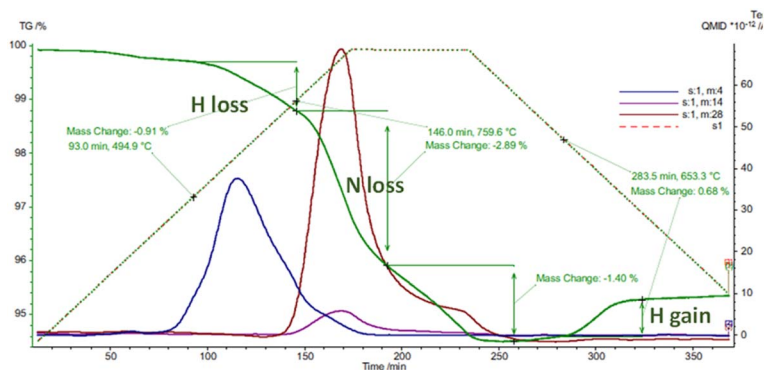
Fig. 6 TGA/MS analysis of a \text{SrND}/\text{Sr}_2\text{ND} sample performed in 5\% \text{H}_2/\text{Ar} showing mass 4, 14 and 28.
