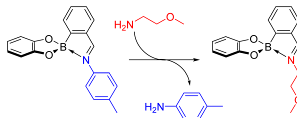
b) Dynamic covalent B–O bonds
