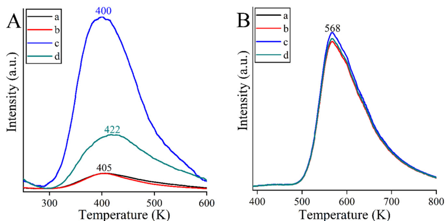
Fig. 4 \text{CO}_2 -TPD curves (A) and \text{NH}_3 -TPD curves (B) of the bismutite-based composites: \text{Bi}_2\text{O}_2\text{CO}_3 (a), \text{MnBi}_2\text{O}_2\text{CO}_3 (b), \text{CoBi}_2\text{O}_2\text{CO}_3 (c) and \text{NiBi}_2\text{O}_2\text{CO}_3 (d).
