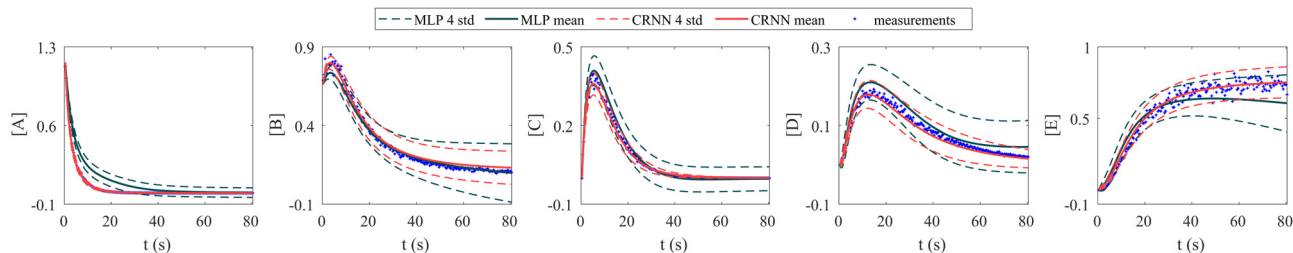
Fig. 9 Uncertainty quantification comparisons between the CRNN and an MLP (without physical laws embedded). Measurements contain 5% Gaussian noise.
