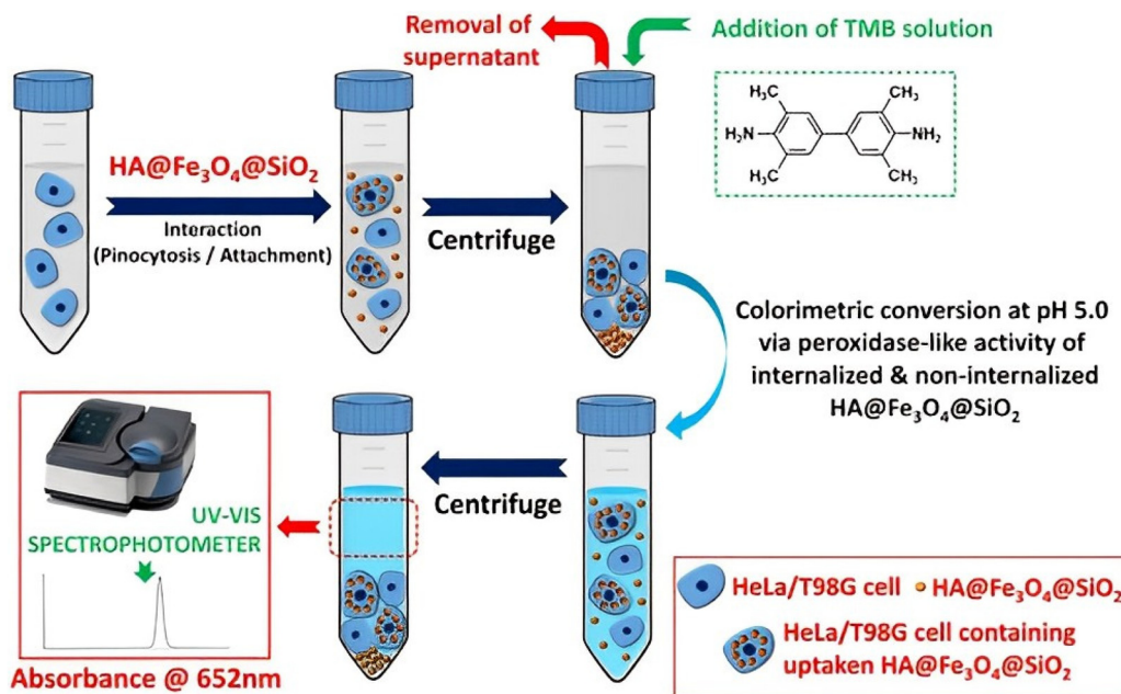
Fig. 5 A schematic diagram for colorimetric determination of HeLa and T98G cell concentrations based on the difference in peroxidase-mimicking activity of HA@Fe 3 O 4 @SiO 2 nanozymes. 93
