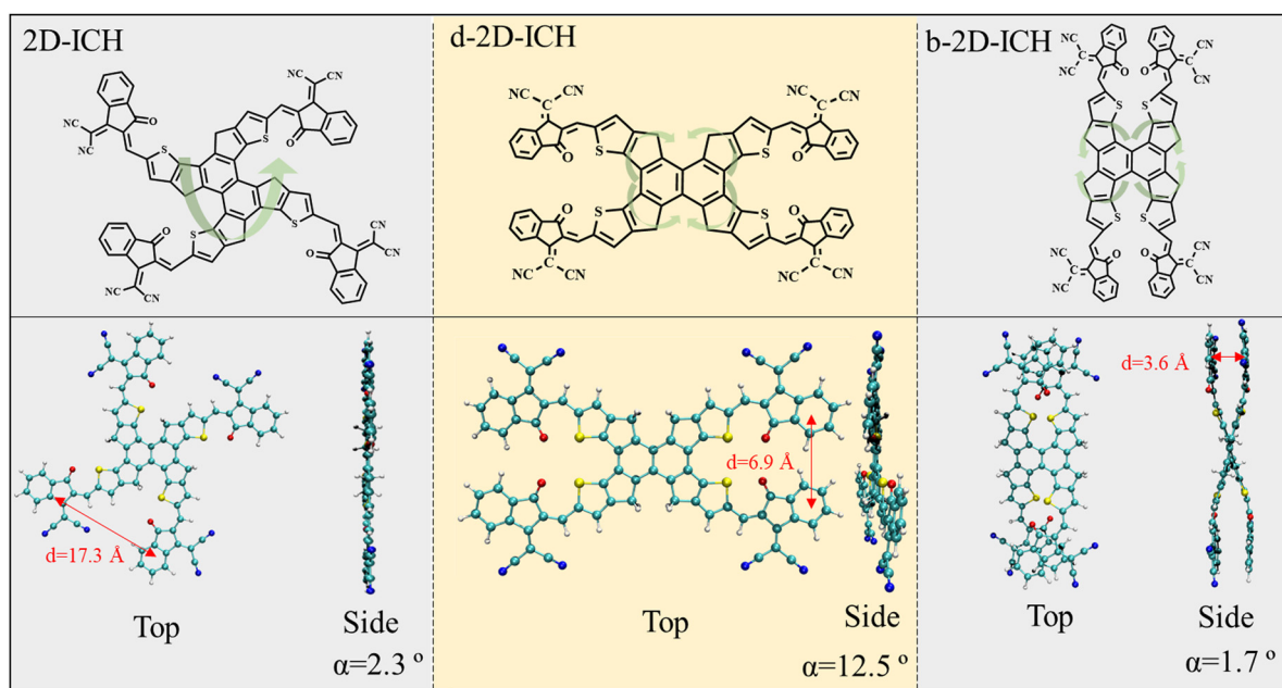
Fig. 1 Chemical structures and top/side view for the optimized structures of 2D-ICH , d-2D-ICH , and b-2D-ICH . Dihedral angle ( \alpha ) and center distance ( d ) of the nearest adjacent end groups are listed at the bottom.
