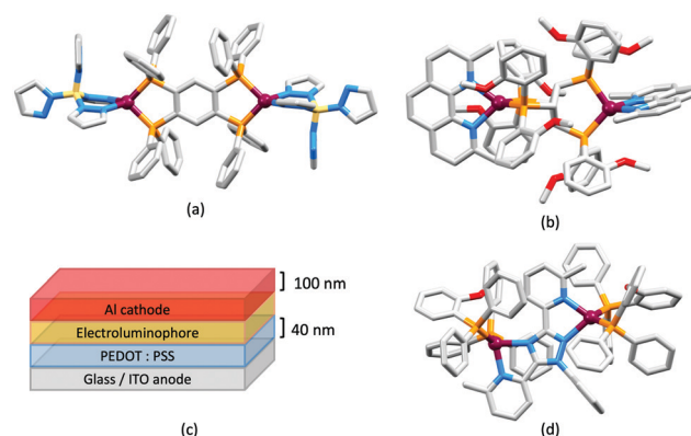
Fig. 22 Structures of (a) [\text{Cu}_2(\text{pz}_4\text{B})_2(\mu\text{-tpbz})] (CSD refcode KURCAD), and (b) the cationic complex in [\text{Cu}_2(2,9\text{-Me}_2\text{phen})_2(\mu\text{-MeOdpccb})][\text{PF}_6]_2 (refcode VOZQAE). (c) Architecture of a LEC containing [\text{Cu}_2(2,9\text{-Me}_2\text{phen})_2(\mu\text{-MeOdpccb})][\text{PF}_6]_2 in the active layer; the LEC was driven under a bias of 4 or 5 V. (d) Structure of the dinuclear cation in [\text{Cu}_2(\text{POP})_2(\mu\text{-37})][\text{BF}_4]_2 (refcode MAMXUW). H atoms are omitted from the figures for clarity.
