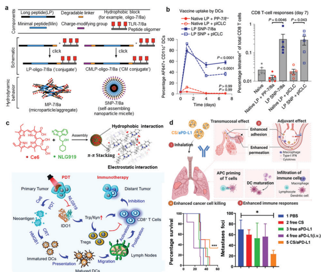
Fig. 2 (a) A nanovaccine platform (SNP-7/8a) based on peptide–TLR-7/8a conjugates that are chemically programmed to self-assemble into micelles. (b) The percentage of total CD11c + DCs that had taken up vaccine (left) and CD8 + T cell responses from blood assessed by tetramer staining (right). 82 Copyright 2020, Springer Nature. (c) Ce6 and NLG919 self-assembled into uniform nanosized particles through hydrophobic, \pi - \pi stacking, and electrostatic interactions and the proposed mechanism for photodynamic sensitized immunotherapy. 88 Copyright 2020, American Chemical Society. (d) Schematic depiction of inhaled CS/aPD-L1 nanoparticles to suppress lung metastases (top), survival curves and numbers of lung metastatic foci after different treatments (bottom). 65 Copyright 2021, John Wiley and Sons.
