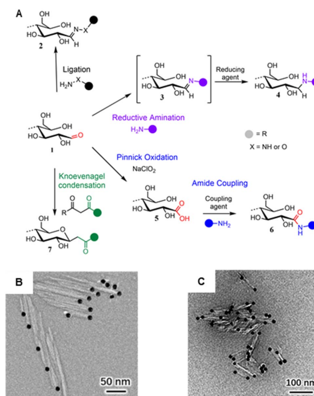
Fig. 8 (A) Main mechanisms used to target cellulose REGs (1): Ligation of hydrazine (NH 2 -NH-R) or hydroxylamine derivatives (NH 2 -O-R) affording hydrazones or oximes (2); reductive amination forming an imine intermediate (3) that is reduced to a stable secondary amine (4); Pinnick oxidation affording carboxylated REGs (5) that allow for subsequent amidation (6); Knoevenagel condensation affording a C-glycoside ketone (7). (B) Asymmetric thioureation of the reducing ends of CNCs during which the aldehyde groups are converted into imine groups, and TEM images of CNC (left) and CNC-II (right) are modified with gold nanoparticles. (A) was adapted with permission from Heise et al. 165 under CC BY 4.0. Copyright 2020 Wiley. (B) was reprinted from Lin et al. , 166 Copyright 2021, with permission from Elsevier. (C) was reproduced from Lin et al. 167 with permission from Royal Society of Chemistry.
