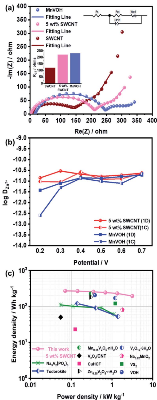
Fig. 5 (a) Nyquist plots of the SWCNT, 5 wt% SWCNT, and MnVOH electrodes. The inset shows a corresponding fitting equivalent circuit, where R_s , R_{ct} , CPE, and W_{01} represent the series resistance, interfacial charge transfer resistance, constant-phase element and Warburg diffusion process, respectively. (b) Comparison of the diffusion coefficient during the first discharge and charge process measured using the PITT method for MnVOH and 5 wt% SWCNTs. (c) Ragone plots compared with different cathode materials for aqueous zinc-ion batteries.
