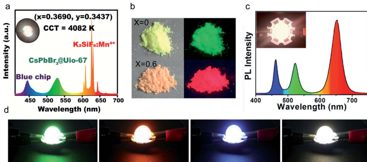
Fig. 8 (a) PL spectra of the as-fabricated WLEDs with the \text{CsPbBr}_3@\text{Uio-67} composite and commercial \text{K}_2\text{SiF}_6:\text{Mn}^{4+} red phosphor deposited on the blue chip (InGaN, 455 nm). Inset: Photograph of the WLEDs. (b) Photographs of \text{CsPbBr}_{3-x}\text{Br}_x/\text{MOF-5} powders ( x = 0 and 0.6 ) taken under daylight (left) and 365 nm UV illumination (right). Reprinted with permission from ref. 113. Copyright 2019 American Chemical Society. (c) The corresponding EL spectrum with a photo of the white LED in the inset. Reprinted from ref. 112. Copyright 2019, with permission from Elsevier. (d) Photograph of blue, green, red, and white LEDs, respectively, using Bio-MOF-1 developed by Zhang et al. Reprinted from ref. 108. Copyright 2019, with permission from Elsevier.
