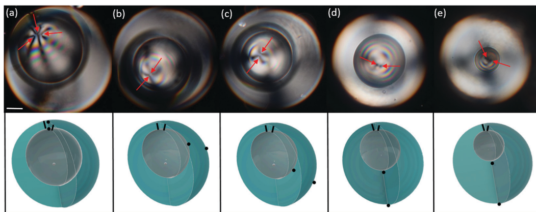
Fig. 4 (a–e) Cross-polarized images of a shell (top view) with one pair of +1 boojums and two +1/2 disclinations at different stages of the de-swelling process. The red arrows indicate the location of the defects. The schematics below (side view) indicate the approximate position of the +1/2 disclinations (black lines spanning the shell thickness) and the +1 boojums (black dots) on the outer sphere and its counterpart on the inner sphere. The time scale of the de-swelling process is of the order of 10 min. Scale bar: 25 \mu\text{m} .
