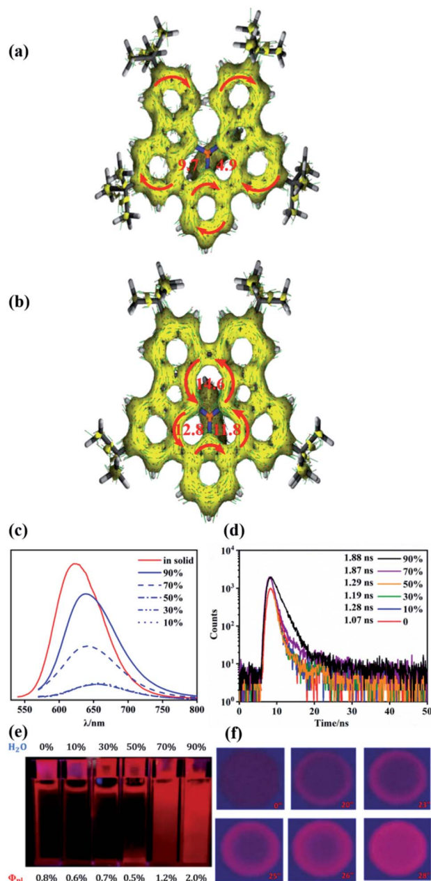
Fig. 6 (a) and (b) ACID plots of NBNN-1 and NBNN-1f , and numbers in red representing NICS(1) in ppm. (c) Emission spectrum change of NBNN-1f in THF with different \text{H}_2\text{O} fractions (vol%). (d) Transient fluorescence curves in THF with different \text{H}_2\text{O} fractions (vol%). (e) Photographs showing the emission intensity increase with increasing \text{H}_2\text{O} fraction. (f) Photographs showing one drop of NBNN-1f solution on a thin-layer chromatography plate with different evaporation timescales.
