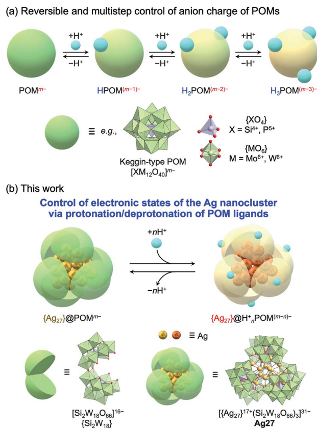
Fig. 1 (a) Control of the anionic charge of polyoxometalates (POMs) via reversible and multistep protonation/deprotonation. (b) This work: control of the electronic states of an \{\text{Ag}_{27}\} nanocluster via protonation/deprotonation of [Si 2 W 18 O 66 ] 16- POM ligands ( \{\text{Si}_2\text{W}_{18}\} ).
