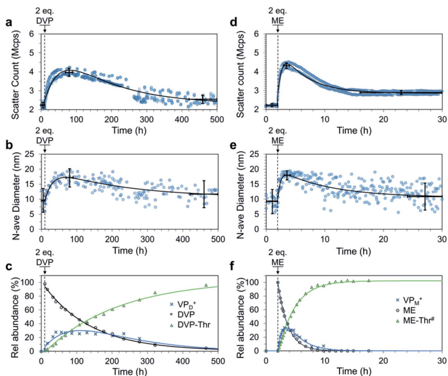
Fig. 6 Fuel-driven transient C3M assembly by addition of 2.0 eq. fuel (DVP or ME) to a solution of P1 (4 mM), PSS (4 mM) and Thr (32 mM for (a–c) and 20 mM for (d–f)). Solutions were maintained at pH 7.4 by 250 mM PB buffer. DLS measurements run in triplicate on independent samples quantitating the scatter count (a and d) and number average diameter (b and e). Two-exponential curves (black line) were fit to the data. Average values (centre of cross) and standard deviation (vertical bars) before fuel addition, at peak micelle assembly and at the end were analysed assuming \sim constant values over the time span shown by the horizontal bars. The process was also monitored by ^1\text{H} NMR (c and f), where only fuel and waste signals were quantitated since PSS was included in the ^1\text{H} NMR experiment. In the case of the ME fuelled experiment multiple waste products were formed, the total of which is described by ME-Thr # . Values for VP D + and VP M + are only an estimate, obtained by subtracting the amount of waste produced from the amount of fuel consumed. The values are expressed as a % conversion of VP in P1. Single and two-exponential curves are drawn to guide the eye. The break in DLS data in figures a and b between 240 and 280 h are due to a required filtration of all samples to remove an unidentified biological growth that began to accumulate in each sample. Filtration was through a 0.45 \mu\text{m} filter and therefore should not significantly remove the \sim 20 nm micelles, for further discussion see Fig. S32 and S33.† Additional DLS, ^1\text{H} NMR and TEM data can be found in Fig. S30–S36.†
