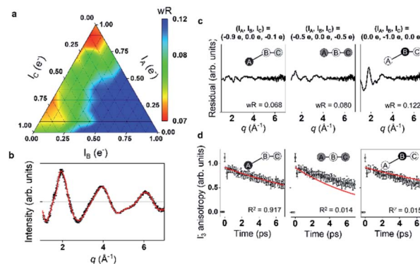
Fig. 9 (a) The weighted R -factors ( wR ) presented as a function of the charges of three I atoms of \text{I}_3^- in methanol determined from a fs-TRXL study. The best fit, which gives the smallest wR , is obtained with I_A = -0.9e , I_B = 0.0e , and I_C = -0.1e . (b) The difference curve at 100 ps (black) and the best fit curve (red) with (I_A, I_B, I_C) = (-0.9e, 0.0e, -0.1e) . (c) Residuals for the differences between the experimental curve and the fit curves obtained for three representative cases of the atomic charge distributions. (d) Comparison of the experimental anisotropy change (black dots with error bars) and the calculated rotational correlation functions (RCFs) for the three representative cases of the atomic charge distributions shown in (c). The coefficient of determination ( R^2 ) for each case is also shown. The best agreement, which gives the lowest wR in (c) and the R^2 value closest to 1 in (d), is found with the first case, providing strong evidence for the localized charge on the terminal iodine atom participating in the longer I–I bond. Reproduced from ref. 93 with the permission of Springer Nature, copyright 2022.
