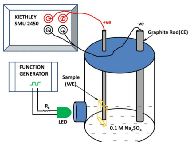
Fig. 27 (a) A representation of the transient surface photovoltage measurement system; (b) measurement of a typical Cu 2 O/FTO electrode in a PEC with 0.1 M Na 2 SO 4 electrolyte followed by real-time measurement in SMU 2450 demonstrating the shape of the LED modulated transient surface photovoltage. 36
