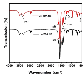
Fig. 4 FTIR spectra of 2D Ln-TDA nanosheets.
