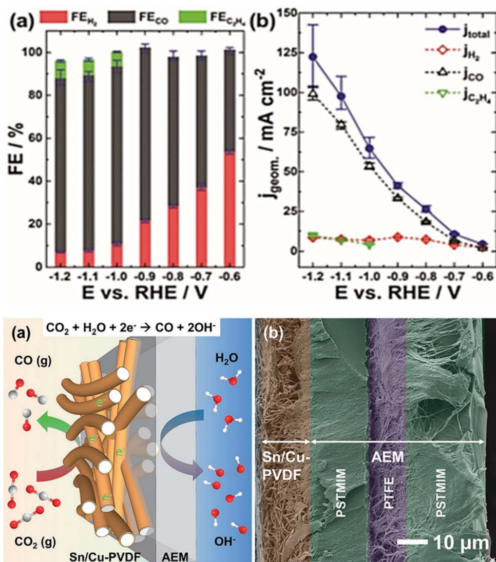
Fig. 2 (Up): (a) Faradaic efficiencies, (b) current densities for electrochemical CO_2 reduction at a Sn/Cu-PVDF GDE at ( -0.6 to -1.2 V vs. RHE). (Bottom): (a) Scheme and (b) cross-sectional SEM image of a Sn/Cu-PVDF/AEM assembly used for electrocatalytic reduction of gaseous CO_2 . Reproduced with permission. 66 Copyright ©2019, Wiley-VCH.
